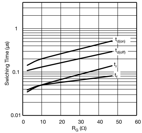
Fig. 12 - Typical MOSFET Switching Time vs. R_G , T_J = 125^\circ\text{C} , I_{DS} = 40\text{ A} , V_{DD} = 250\text{ V} , V_{GS} = 10\text{ V} , L = 500\ \mu\text{H} Diode used 60APH06
