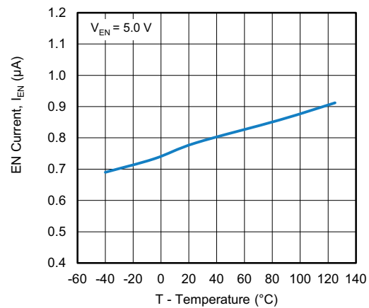
Fig. 26 - EN Current vs. Junction Temperature
