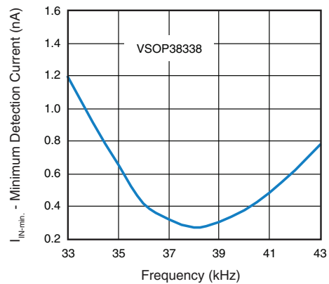
Fig. 4 - Bandpassfilter Characteristic
