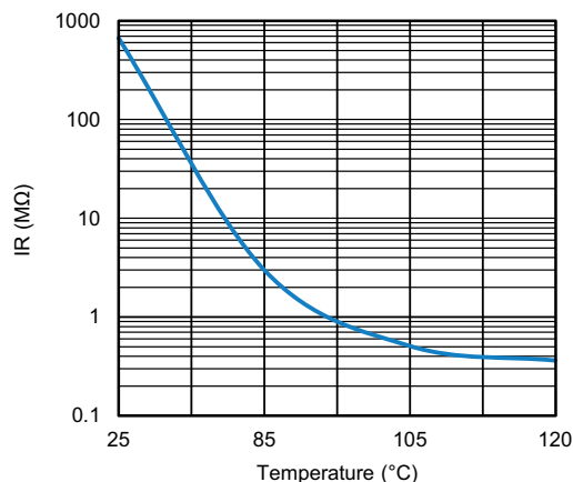
Fig. 5 - IR in function of temperature
