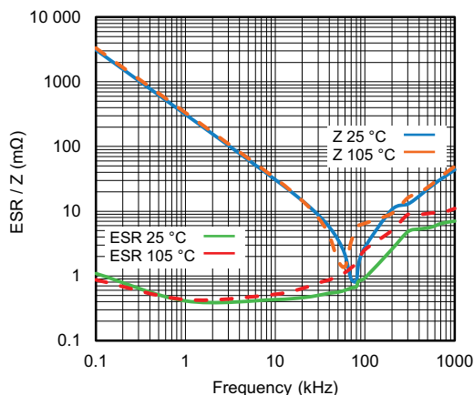
Fig. 2 - ESR and Impedance in function of frequency at different temperatures (MKP1849750090K)
