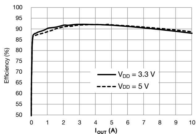
Fig. 6 - PSM Efficiency - V_{DD} 3.3 V vs. 5 V ( V_{OUT} = 1.5\text{ V} , V_{IN} = 12\text{ V} )
