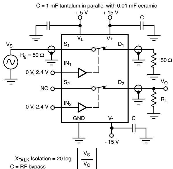
Fig. 4 - Crosstalk
