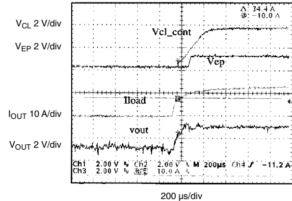
Figure 10. Overload Recovery
