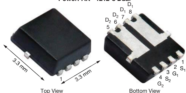
PowerPAK® 1212-8 Dual
