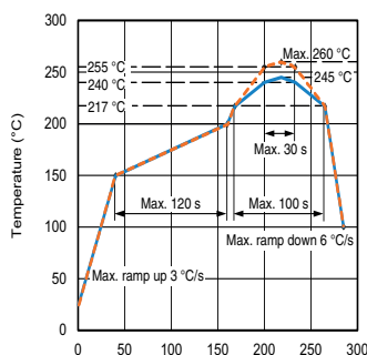
Fig. 10 - Lead (Pb)-free Reflow Solder Profile acc. J-STD-020
