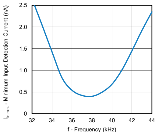
Fig. 4 - Bandpassfilter Characteristic
