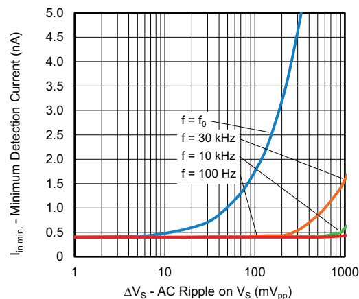
Fig. 5 - Suppression of Ripple on Supply Voltage
