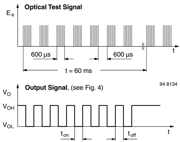
Fig. 3 - Test Signal
