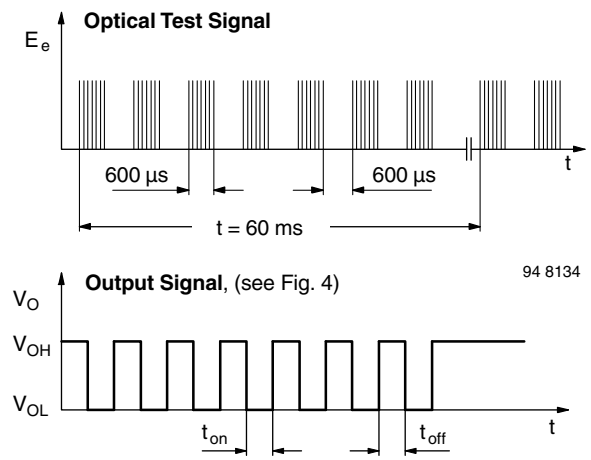
Fig. 3 - Test Signal
