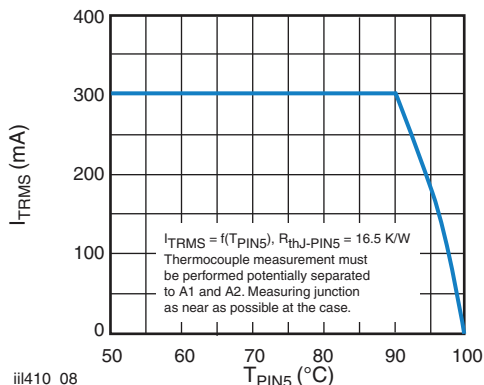
Fig. 6 - Current Reduction
