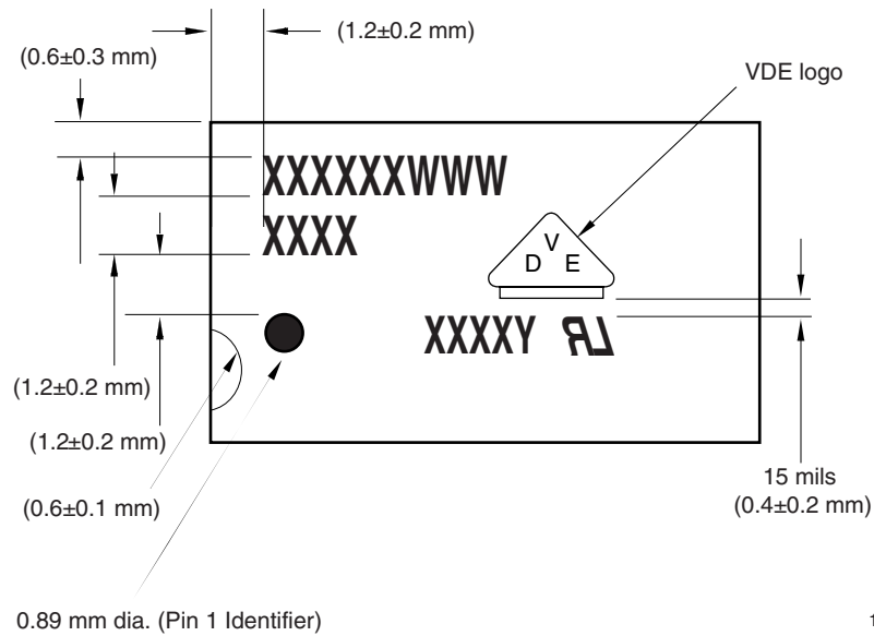
Figure 1. 6-pin and 8-pin SSRs
