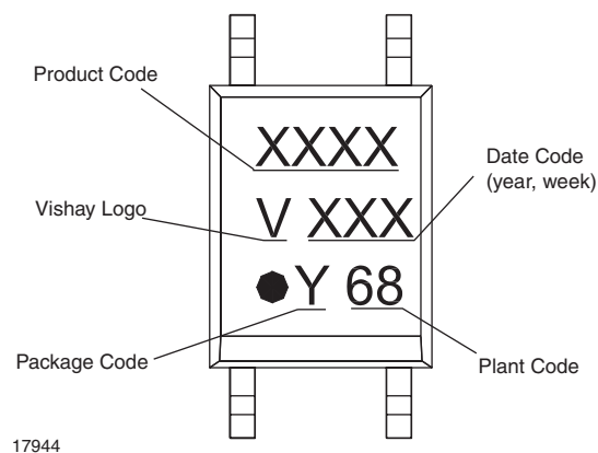
Figure 3. 4-pin SOP
