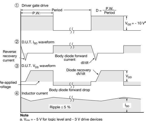
Fig. 19 - For P-Channel
