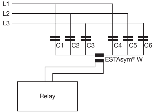
Fig. 1 - Double-star connection
