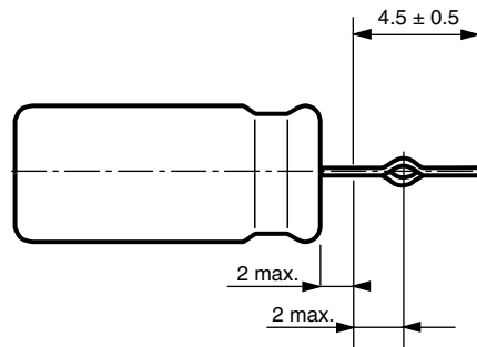
5 \leq \varnothing D \leq Leads bent open, shortened and formed EKS 09... (S = 5 mm)
