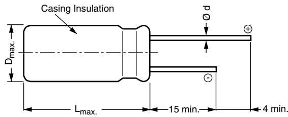
5 \leq \varnothing D \leq 18 Long leads EKS 00...
