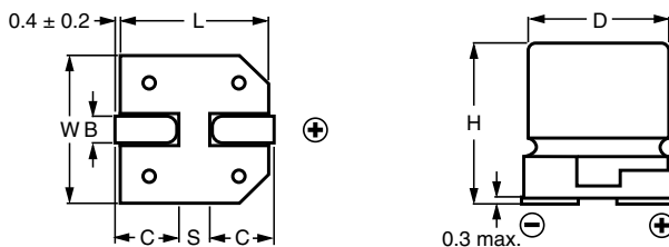
Fig.2 Dimensional outline
