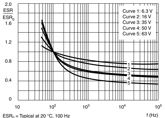
ESR_0 = Typical at 20^{\circ}C , 100 Hz
