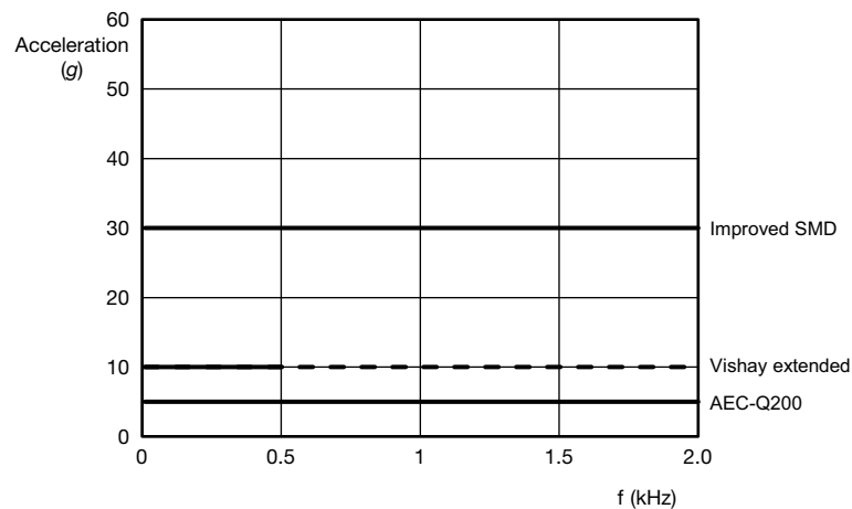
Fig. 5 - Vibration profile
