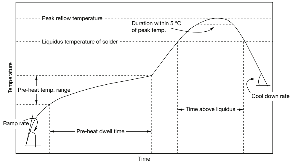
Fig. 1 - Typical Lead (Pb)-Free Reflow Soldering Profile for SMDY1 Series / SMDY1...S Series
