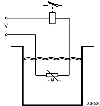
Fig. 9 - Liquid level control
