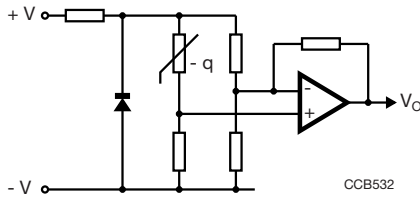
Fig. 11 - Temperature sensing bridge with op-amp which acts as differential amplifier. The sensitivity can be very high
