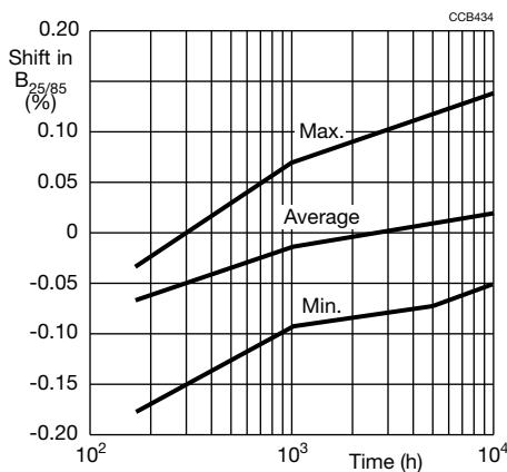
Fig. 3 - Aging characteristics (dry heat at 150 °C of a NTCLE100E3 series NTC temperature sensor with an R_{25} of 10 k \Omega )
