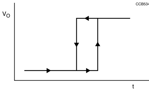
Fig. 13 - Transfer characteristic of the circuit shown in Fig. 12
