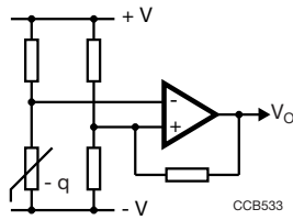
Fig. 12 - Basic temperature sensing configuration. The op-amp acts as a Schmitt-trigger. The transfer characteristic is shown in Fig. 13
