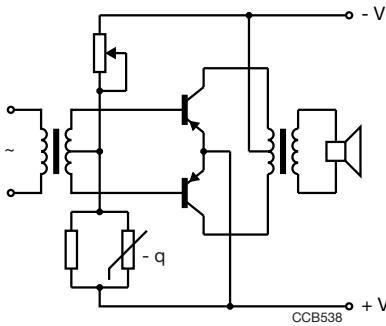
Fig. 17 - Temperature compensation in transistor circuits. Push-pull compensation
