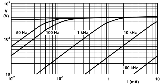
Effect of HF alternating current on varistor type VDRS14T250; C = 480 pF
