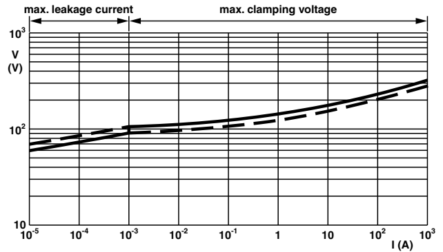
Curve for varistor type VDRS07H060
