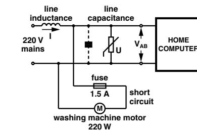
Influence of a transient on the mains voltage
