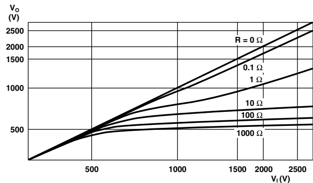
Influence of a series resistance on the varistor
