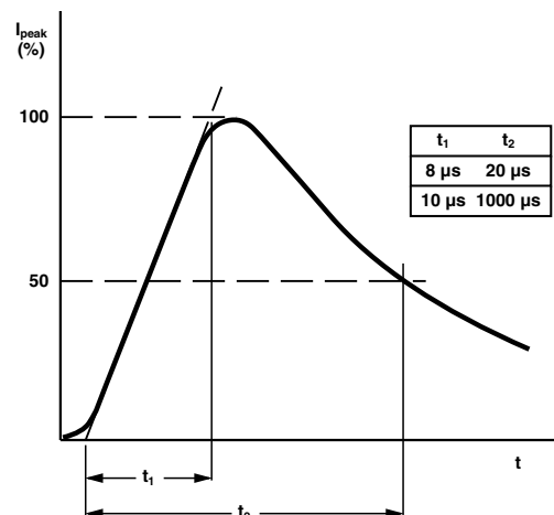
Standard pulse for current and maximum allowable energy calculation
