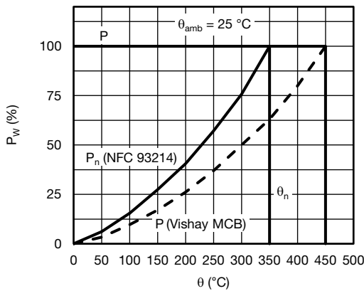
Power P w as a Function of Surface Temperature P(W) = f(\text{Temperature Surface})
