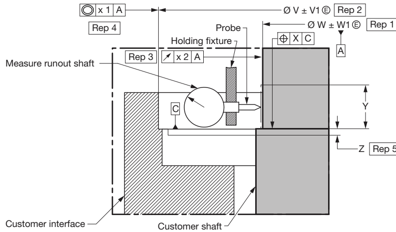
Fig. 1 - Mounting Detail
