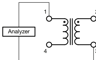
DWV Test (coil to coil)
