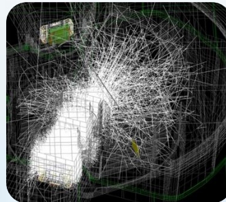
Ray Tracing
