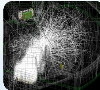
Ray Tracing
