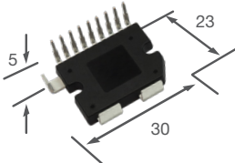
FlatPAK HC0
