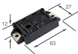
EMIPAK-1B
