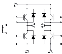
Full Bridge With Thermistor (VS-...MT...TFT)
