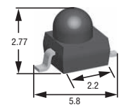
1.8 mm Gullwing
