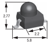
1.8 mm Gullwing
