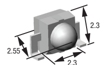
1.8 mm Side-View
