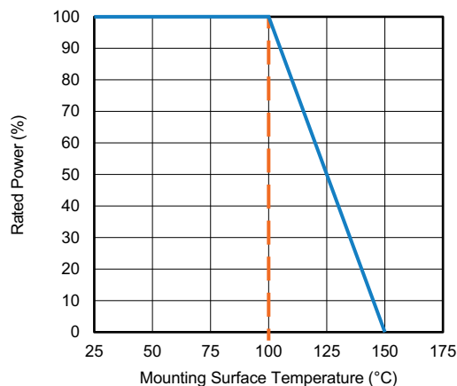
Fig. 3 - Derating Curve
