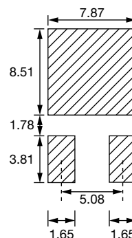
Soldering Pad DTO
