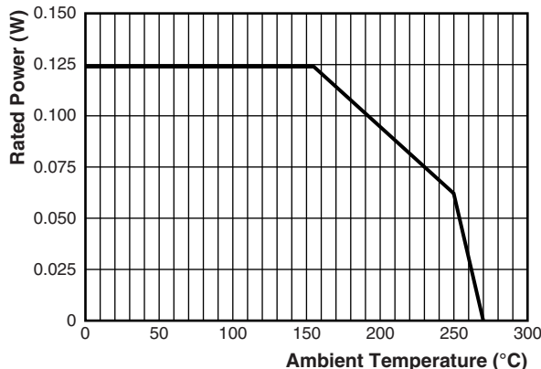
PVHT0603 Power Derating Curve
