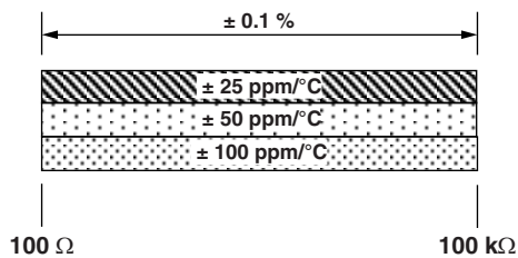
Tightest Standard Tolerance Available
