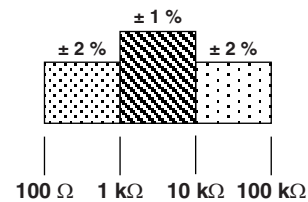
Load Life Stability, 1000 h, +125 °C, 175 mW
