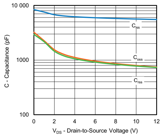
Capacitance a
