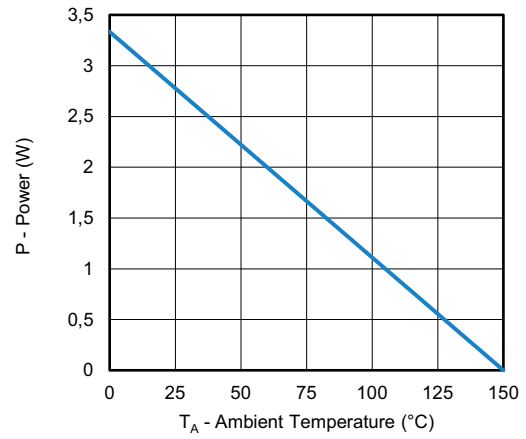
Power Derating
