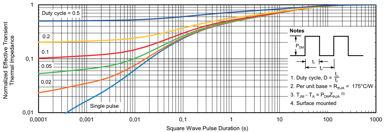
Normalized Thermal Transient Impedance, Junction-to-Ambient (1" x 1" FR4 Board with Minimum Copper)
