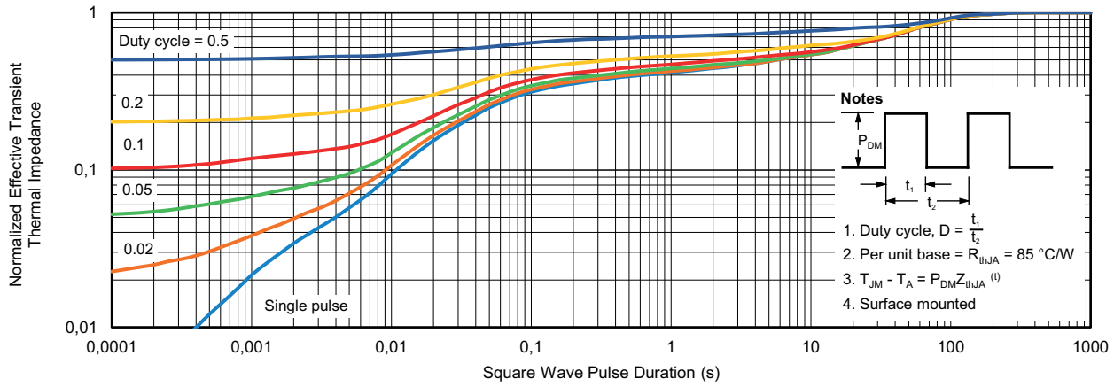
Normalized Thermal Transient Impedance, Junction-to-Ambient (1" x 1" FR4 Board with Full Copper)
