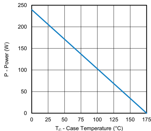
Power, Junction-to-Case
