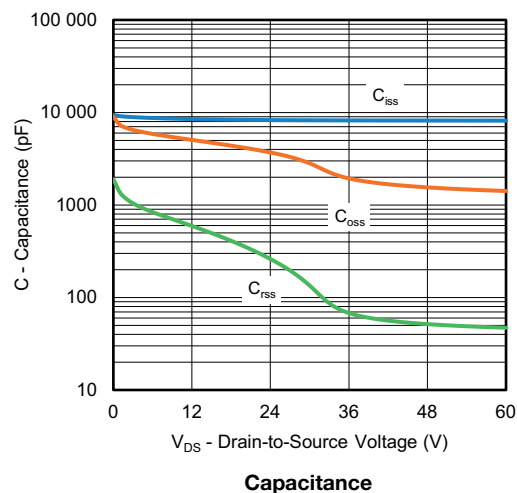
Capacitance
