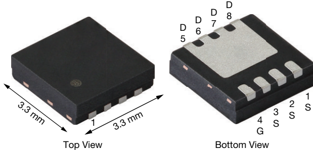
PowerPAK® 1212-8SLW
