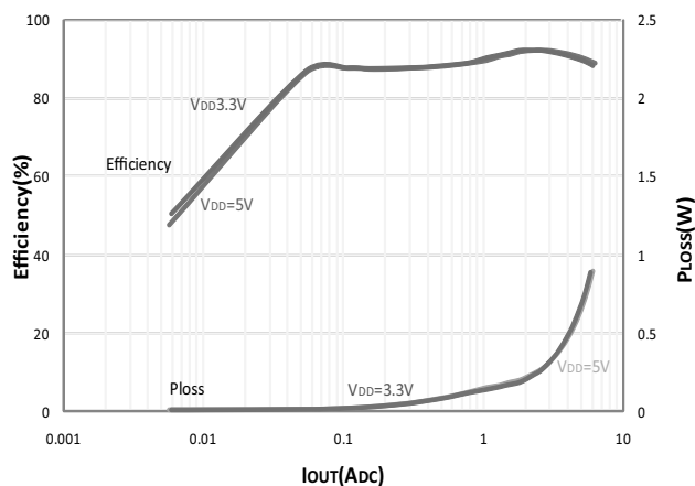
Efficiency vs. Load-PSAVE Mode V_{OUT} = 1.2\text{ V} , V_{IN} = 12\text{ V} , V_{DD} = \text{EN/PSV} = 5\text{ V} , External Bias, SiC403A
