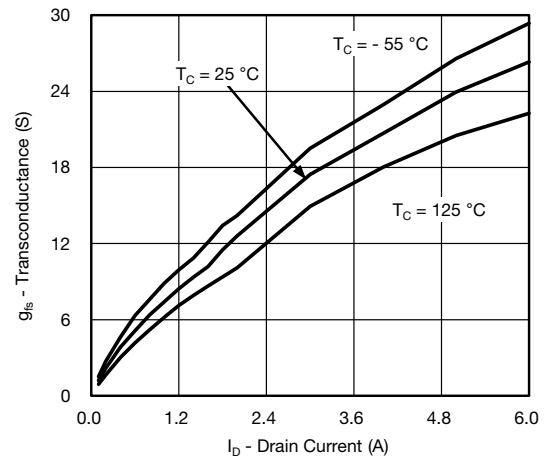
Transconductance
