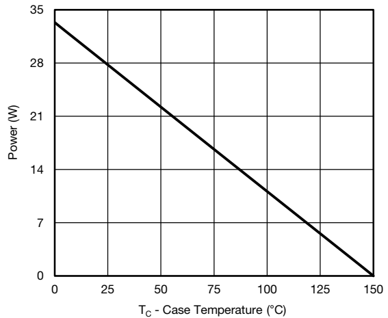
Power, Junction-to-Case
