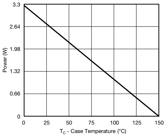
Power, Junction-to-Foot
