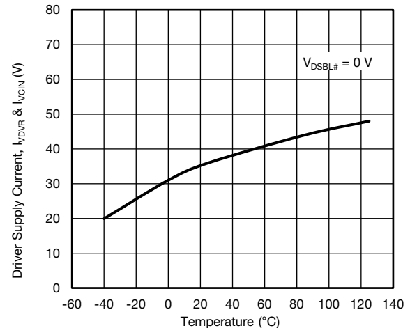
Fig. 22 - Driver Shutdown Current vs. Temperature
