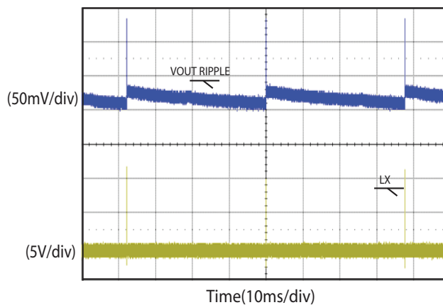
Power-Save Mode ( V_{DD} = 5\text{ V} , V_{IN} = 12\text{ V} , V_{OUT} = 1.5\text{ V} , I_{OUT} = 0\text{ A} , SiC401B)
