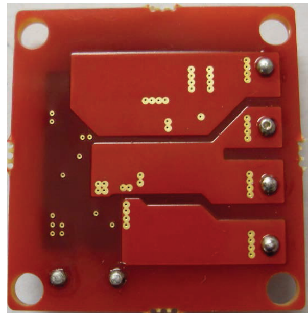
Fig. 2 - Bottom of the PCB
