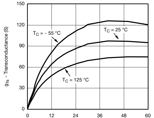
Transconductance
