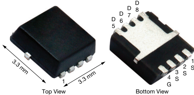
PowerPAK® 1212-8 Single
