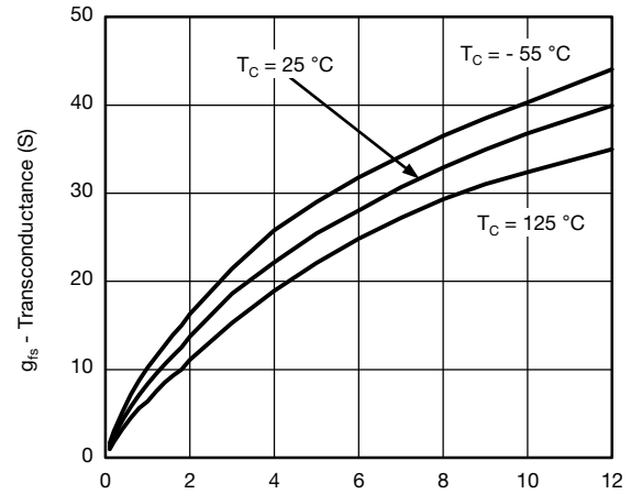
I_D - Drain Current (A) Transconductance
