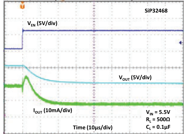
Fig. 36 - Turn-off Time
