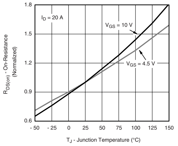
I_D = 20\text{ A} V_{GS} = 10\text{ V} V_{GS} = 4.5\text{ V} On-Resistance vs. Junction Temperature
