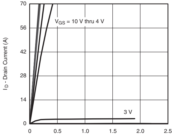
V_{GS} = 10 V thru 4 V Output Characteristics
